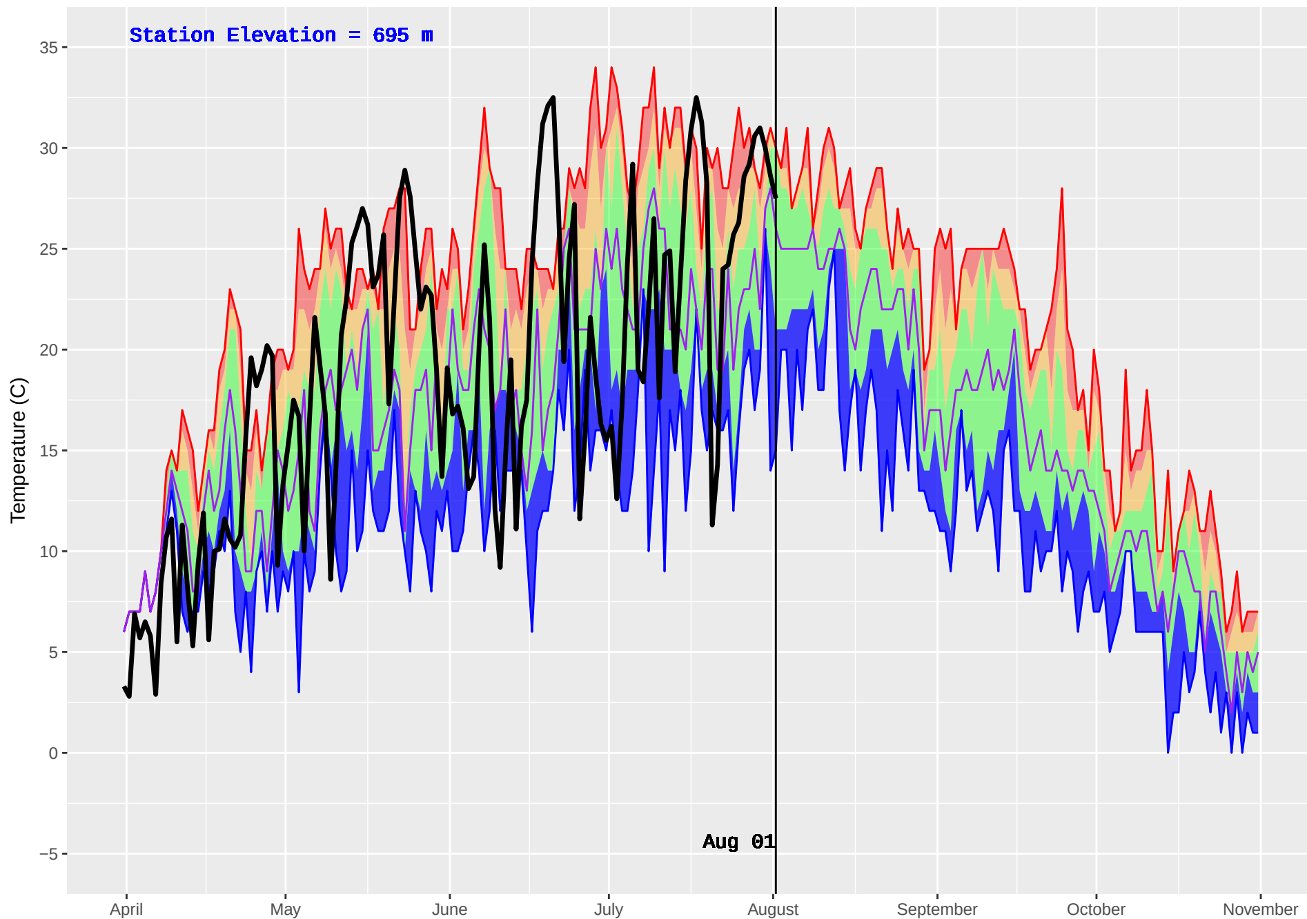
BLUE RIVER 2 (1108) : Historical (2011–2016) and Current (2018) Daily Temperature
