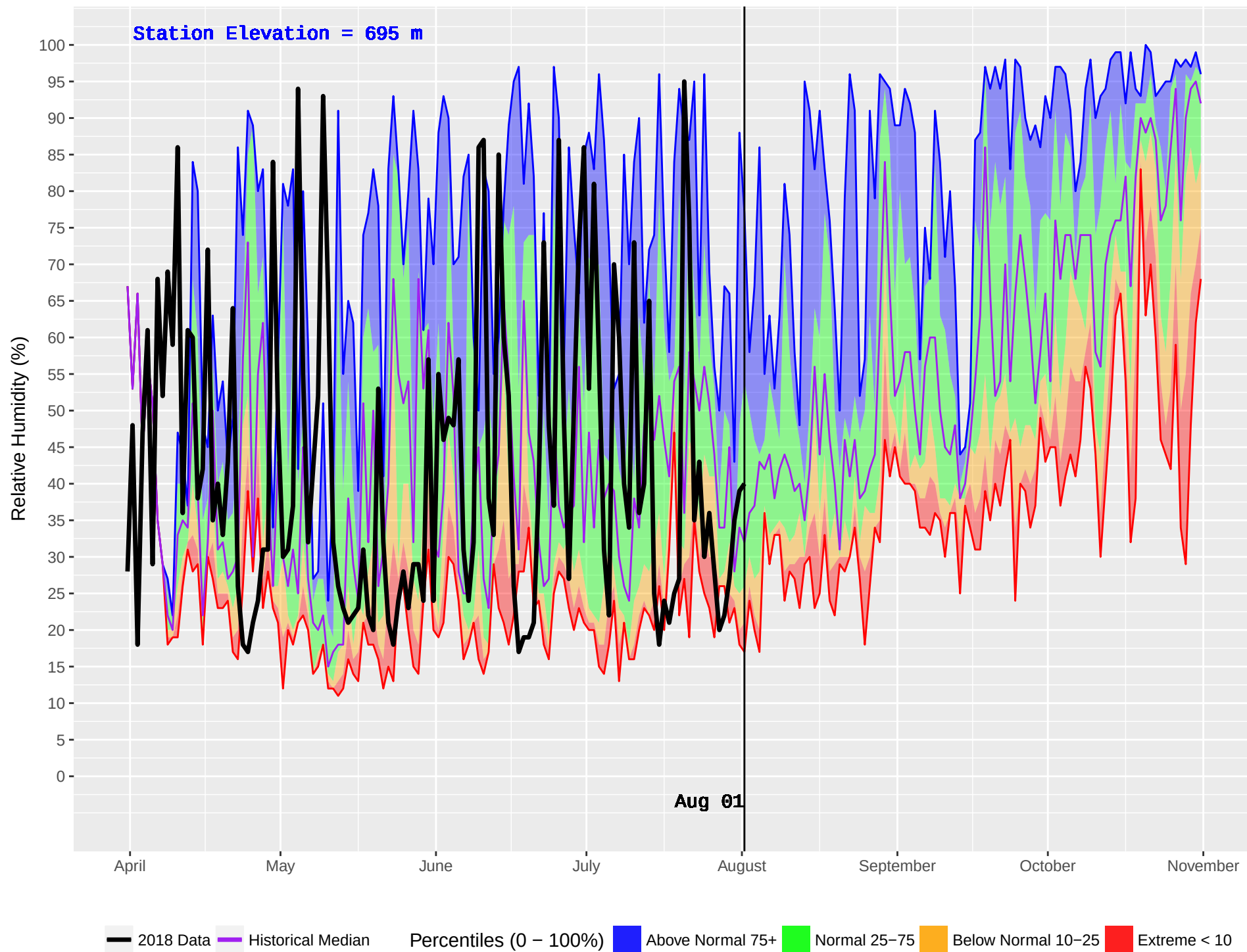
BLUE RIVER 2 (1108) : Historical (2011–2016) and Current (2018) Daily Relative Humidity
