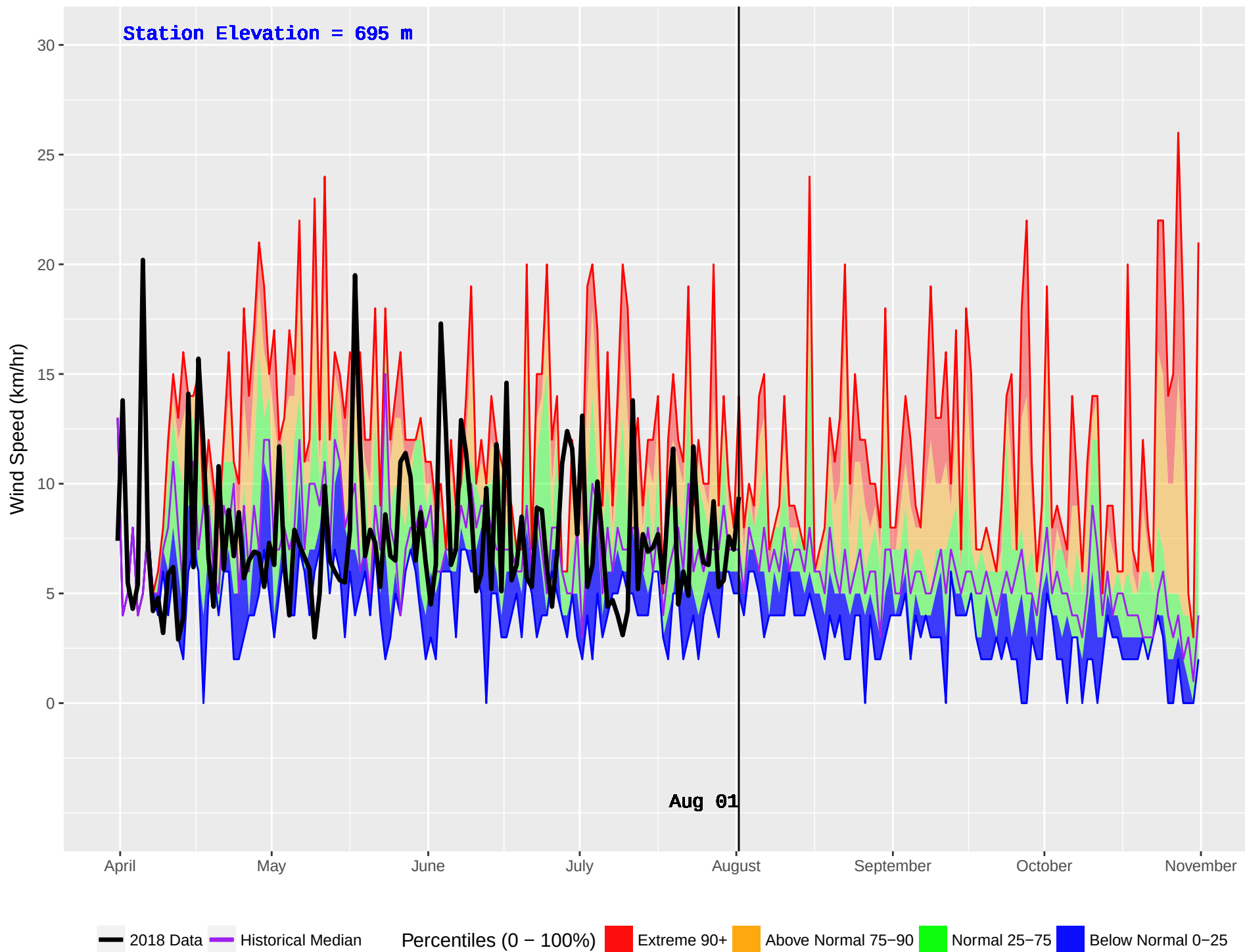
BLUE RIVER 2 (1108) : Historical (2011–2016) and Current (2018) Daily Wind Speed
