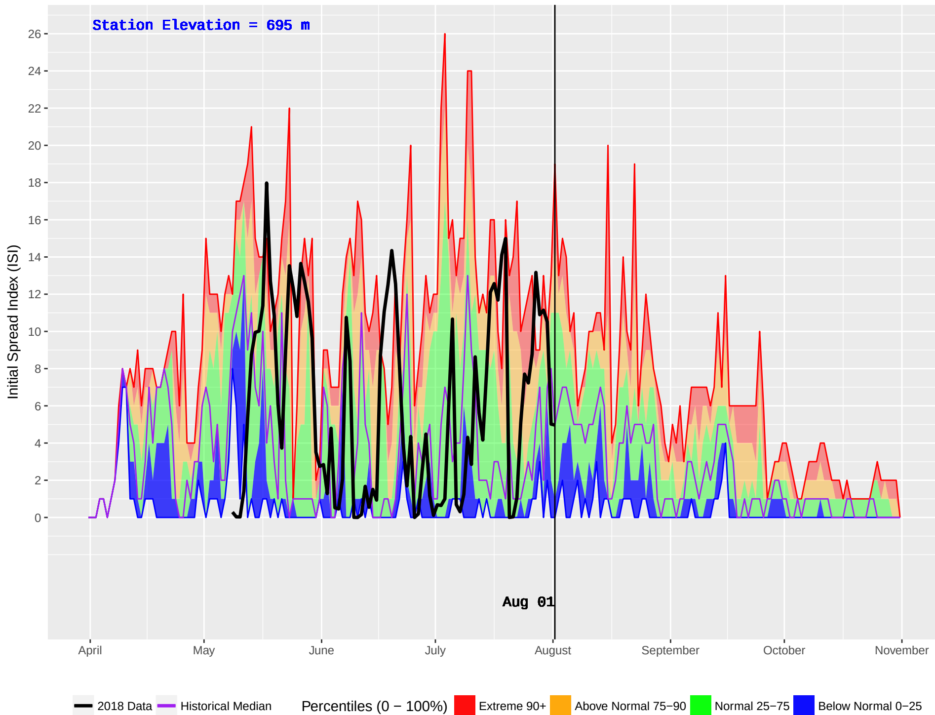
BLUE RIVER 2 (1108) : Historical (2011–2016) and Current (2018) Daily Initial Spread Index (ISI)
